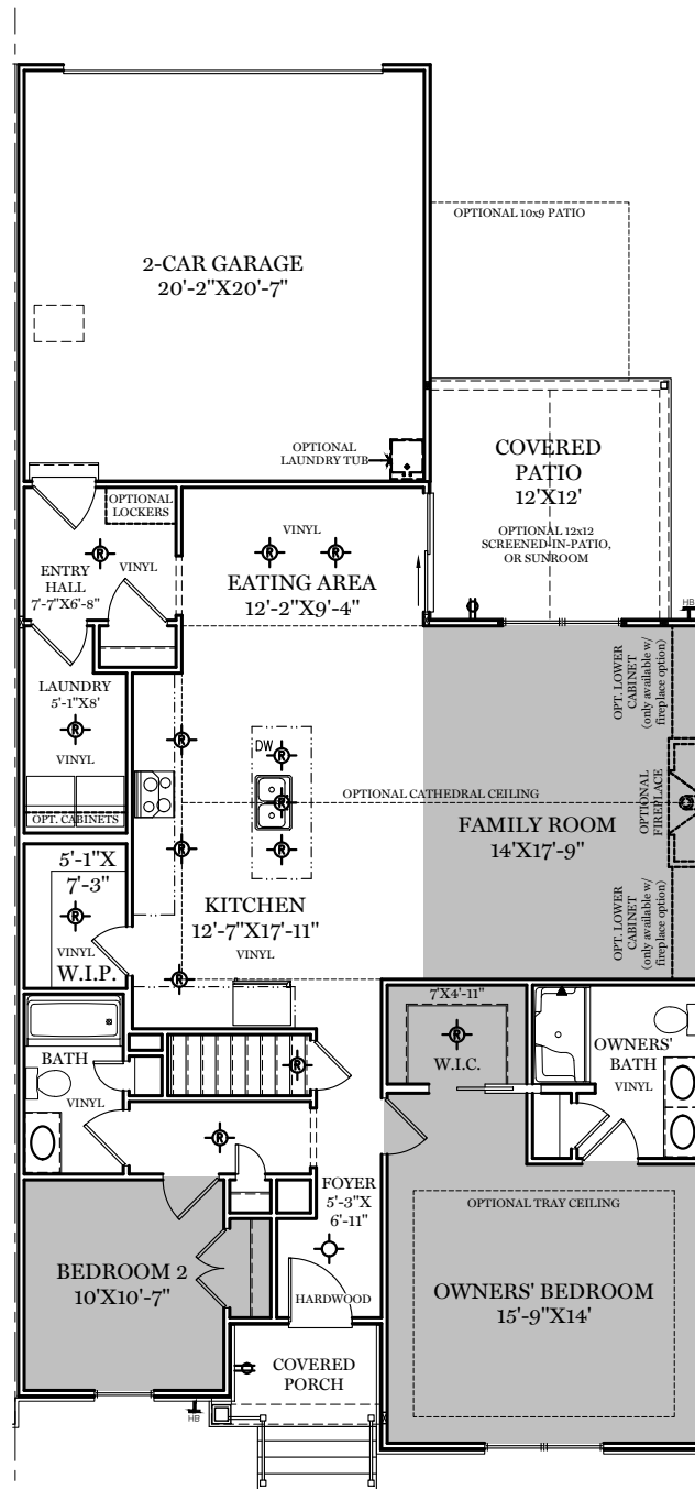
1st Floor Plan - 1,541 sf STONECROFT I
